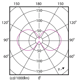
Light Distribution Diagram - CLA LEDLuster ND 4-40W P45 E27 827 CL
