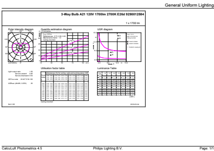
General uniform lighting - 22A21/LED/827 3WAY ND 120V 6/1
