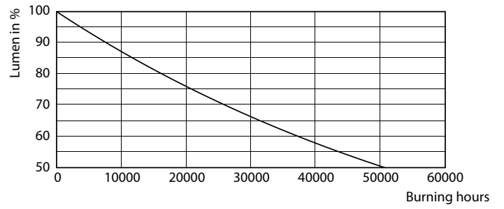
Lumen Maintenance Diagram - 8A19/LED/827/ND D2D 120V 6/1
