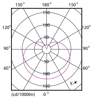
Light Distribution Diagram - 8A19/LED/827/ND D2D 120V 6/1
