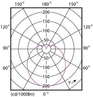
Light Distribution Diagram - LED SSW 60W A60 E27 WW-CW FR ND 1BC/4
