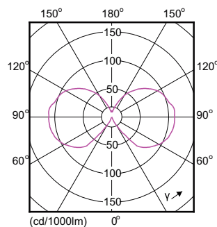
Light Distribution Diagram - CLA LEDBulb DT 4.5-40W A60 E27 CL
