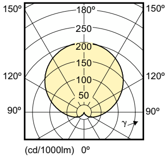
Light Distribution Diagram - ESS LEDBulb 6-42W E27 6500K 230V A60 TR
