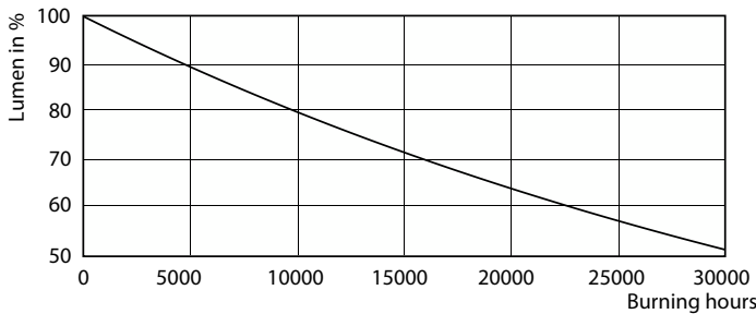
Lumen Maintenance Diagram - LEDClassic 5-50W MR16 830 60D
