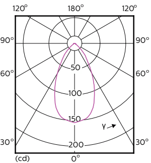
Light Distribution Diagram - LEDClassic 5-50W MR16 830 60D
