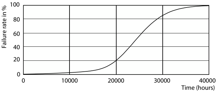
Life Expectancy Diagram - LEDClassic 5-50W MR16 830 60D
