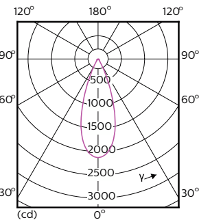
Light Distribution Diagram - 12PAR30S/EXPERTCOLOR RETAIL/F40/930/DIM
