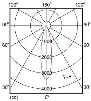
Light Distribution Diagram - 12PAR30L/AMB/F25/827/DIM ULW
