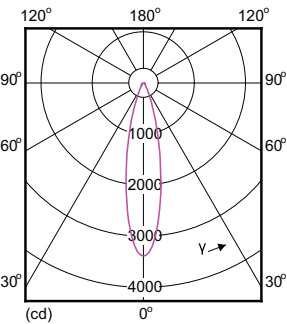
Light Distribution Diagram - 12PAR30L/AMB/F25/830/DIM ULW
