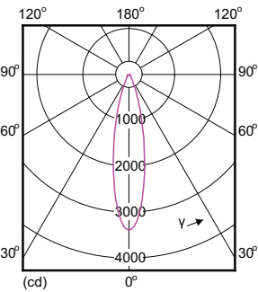
Light Distribution Diagram - 12PAR30S/AMB/F25/827/DIM ULW
