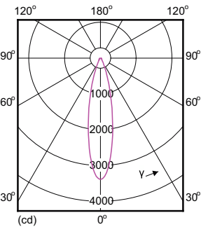
Light Distribution Diagram - 12PAR30S/AMB/F25/830/DIM ULW
