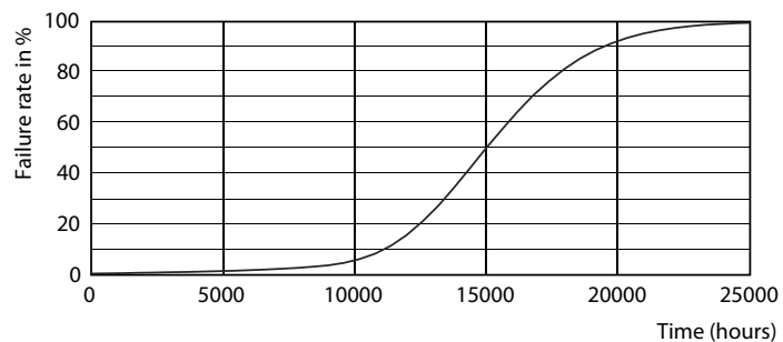
Life Expectancy Diagram - CLA LEDspotMV ND 520lm GU10 830 120D
