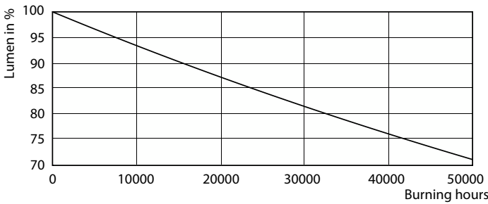
Lumen Maintenance Diagram - MAS LEDtube 1500mm UO 24W 830 T8
