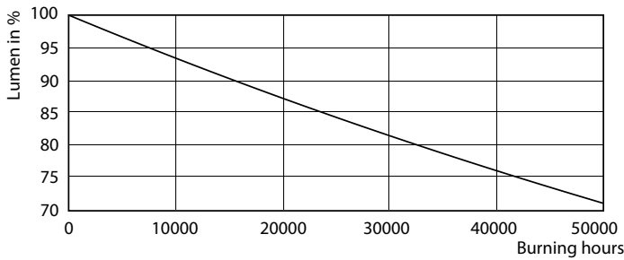
Lumen Maintenance Diagram - MAS LEDtube 1500mm UO 24W 840 T8
