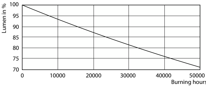
Lumen Maintenance Diagram - MAS LEDtube 1500mm HO 20W840 T8
