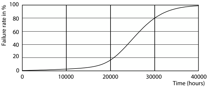
Life Expectancy Diagram - 4.5GU10/LEDCLA/F35/830/DIM 10/1
