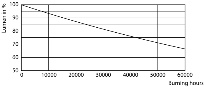
Lumen Maintenance Diagram - 14T8/48-4000 IF 10/1 ROT
