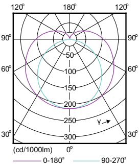
Light Distribution Diagram - 14T8/48-4000 IF 10/1 ROT
