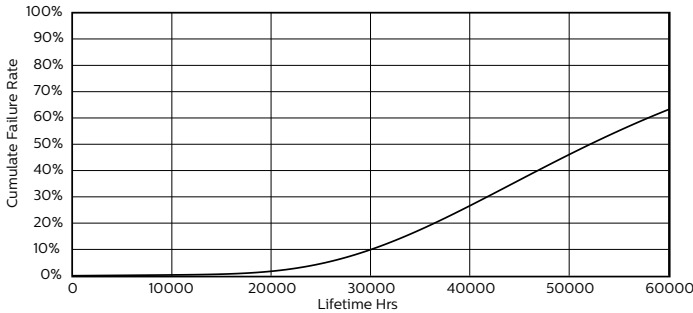
Life Expectancy Diagram - 14T8/48-4000 IF 10/1 ROT
