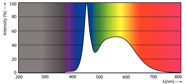
Spectral Power Distribution Colour - LEDBulb 8-70W E27 865 220-240V 2BL/4
