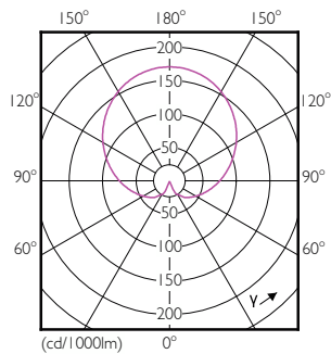
Light Distribution Diagram - LEDBulb 8-70W E27 865 220-240V 2BL/4
