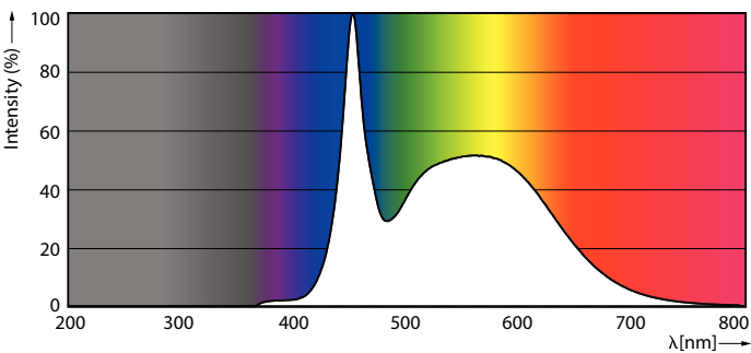
Spectral Power Distribution Colour - LEDBulb 8-70W E27 865 220-240V 3PF/4
