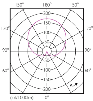
Light Distribution Diagram - LEDBulb 8-70W E27 865 220-240V 3PF/4
