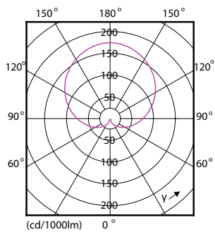
Light Distribution Diagram - CorePro LEDbulb ND 12.5-100W A60 E27 865
