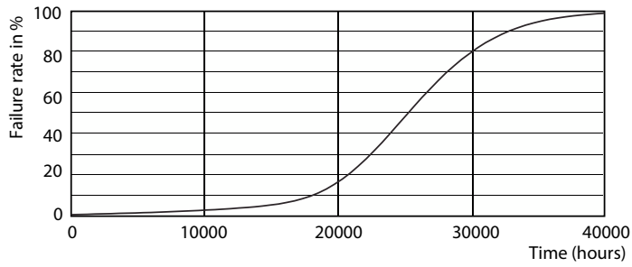
Life Expectancy Diagram - 7PAR20/LED/F40/830/E26/GL/DIM 120V
