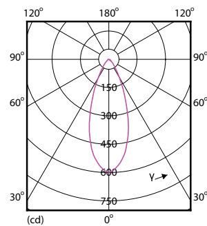
Light Distribution Diagram - 7PAR20/LED/F40/840/E26/GL/DIM 120V
