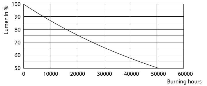
Lumen Maintenance Diagram - 7PAR20/LED/F40/840/E26/GL/DIM 120V
