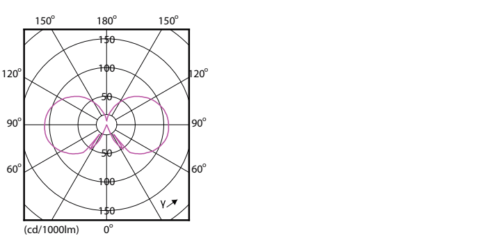
Light Distribution Diagram - CLA LEDLuster D 2.7-25W P45 E27 827 CL
