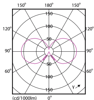
Light Distribution Diagram - CLA LEDCandle D 5-40W BA35 E14 827 CL
