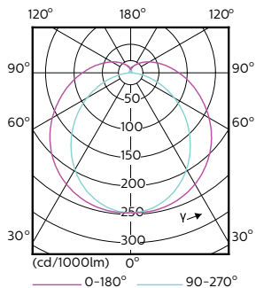
Light Distribution Diagram - MAS LEDtube UN 1500mm UO 24W830 T8
