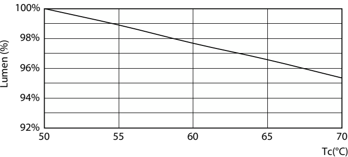
Lumen Maintenance Diagram - CorePro LEDtube 600mm 8W840
