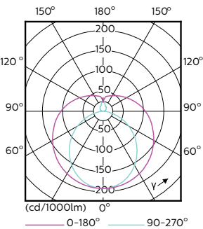
Light Distribution Diagram - CorePro LEDtube 600mm 8W840
