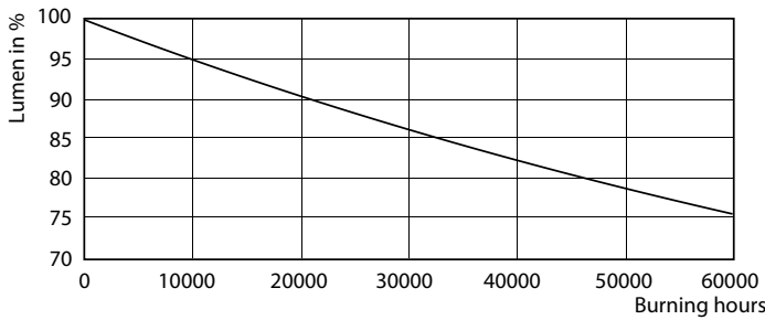
Lumen Maintenance Diagram - MAS LED ExpertColor 6.5-35W MR16 927 60D
