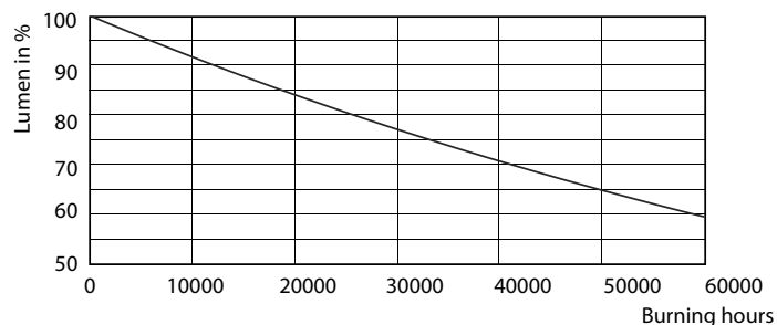
Lumen Maintenance Diagram - MAS LED ExpertColor 6.5-35W MR16 940 36D
