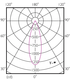
Light Distribution Diagram - MAS LED ExpertColor 6.5-35W MR16 940 36D
