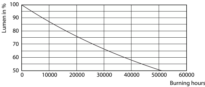
Lumen Maintenance Diagram - MAS LED spot VLE D 680lm GU10 840 120D
