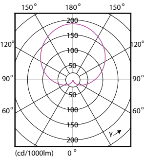
Light Distribution Diagram - CorePro LEDbulb D 11-75W A60 E27 827
