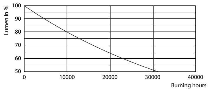
Lumen Maintenance Diagram - CorePro LEDbulb D 5.5-40W A60 B22 827
