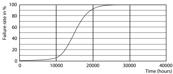
Life Expectancy Diagram - CorePro LEDbulb D 5.5-40W A60 B22 827
