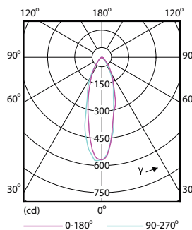
Light Distribution Diagram - CorePro LEDspot 4-35W GU10 827 36D DIM
