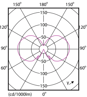
Light Distribution Diagram - CLA LEDBulb ND 8-75W E27 CW A60 CL
