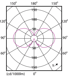
Light Distribution Diagram - CLA LEDBulb ND 11-100W E27 CW A67 CL
