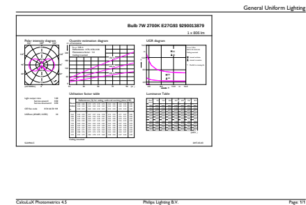
General uniform lighting - CLA LEDBulb ND 7-60W E27 WW G93 CL
