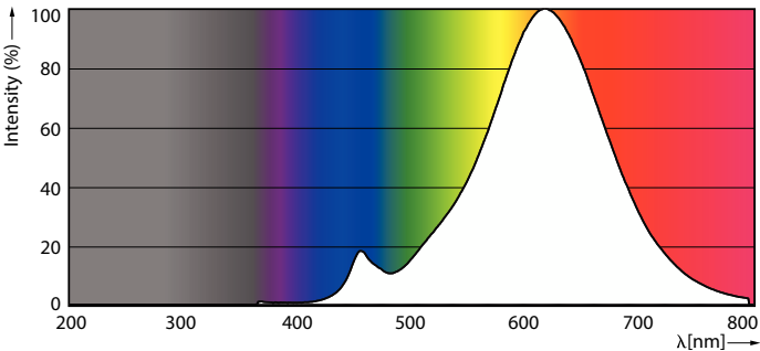
Spectral Power Distribution Colour - CLA LEDBulb ND 7-60W E27 WW G93 CL
