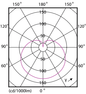
Light Distribution Diagram - CorePro lustre ND 5.5-40W E14 865 P45 FR
