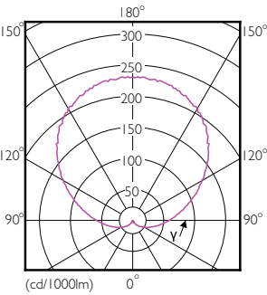
Light Distribution Diagram - Ess LEDBulb 3.5-25W E27 3000K A19 1PK MX
