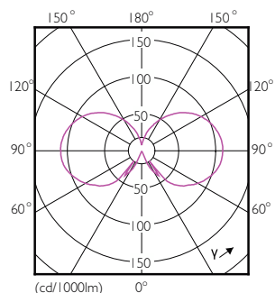
Light Distribution Diagram - CLA LEDCandle D 5-32W B35 E14 822 GOLD
