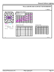
General uniform lighting - TForce LED HPL ND 44-33W E27 740 FR
