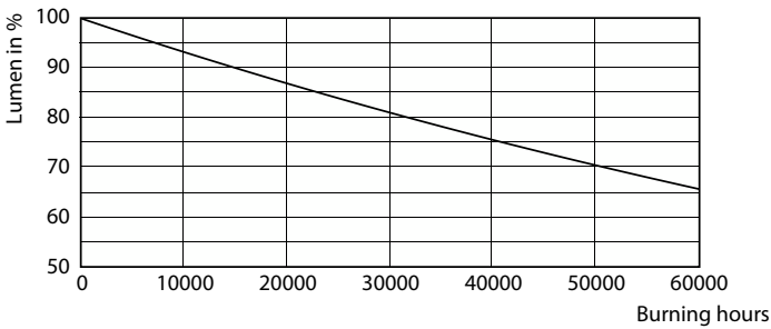
Lumen Maintenance Diagram - TForce LED HPL ND 44-33W E27 740 FR
