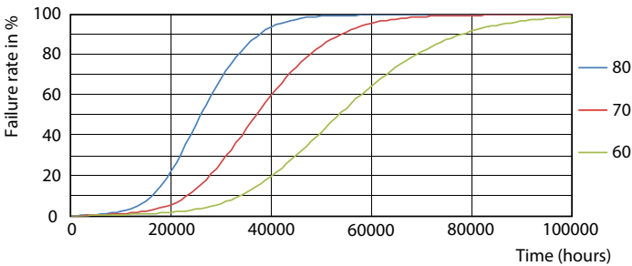
Life Expectancy Diagram - MAS LEDtube 1500mm UO 24W 840 T8 G
