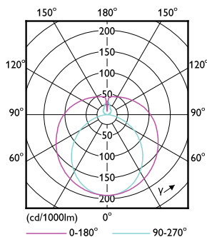
Light Distribution Diagram - MAS LEDtube 1500mm UO 24W 840 T8 G
