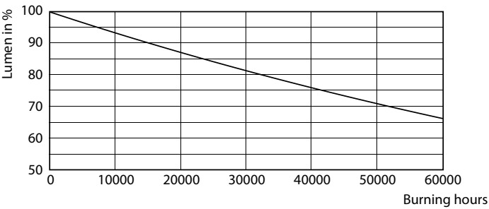
Lumen Maintenance Diagram - MAS LEDtube 1500mm UO 24W 840 T8 G
