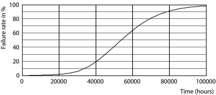
Life Expectancy Diagram - MAS LEDtube 1500mm UO 24W 840 T8 G
