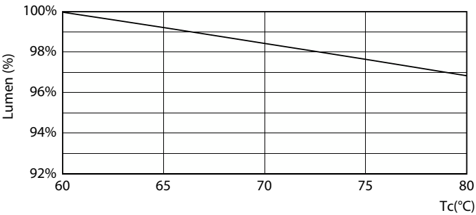
Lumen Maintenance Diagram - MAS LEDtube 1500mm UO 24W 840 T8 G
