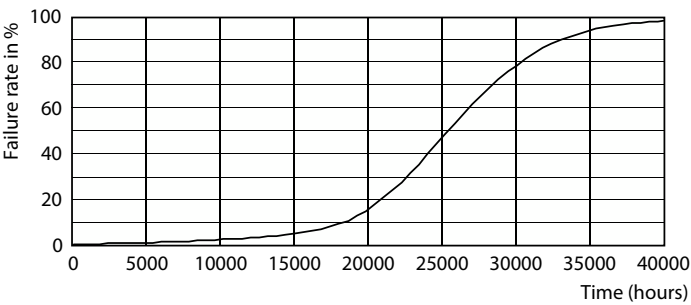
Life Expectancy Diagram - TForce Core LED PT 30-27W E27 830 FR
