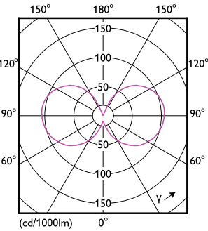
Light Distribution Diagram - CorePro LEDLusterND6.5-60W P45 E27827CLG
