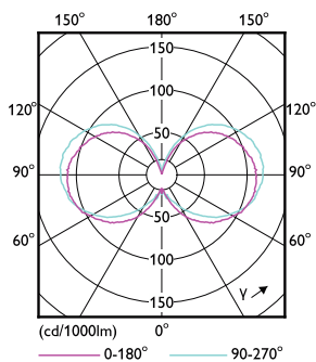
Light Distribution Diagram - CLA LEDBulb D 7.2-60W G95 E27 827 CL
