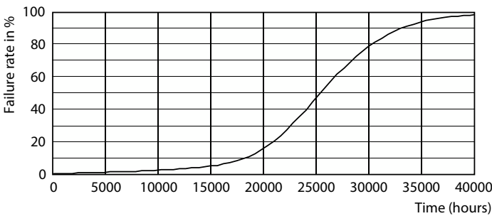
Life Expectancy Diagram - TForce Core LED road 40W 740 E40 MV
