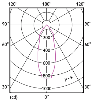
Light Distribution Diagram - RS060B LED5-36/830 PSR II WH LILO
