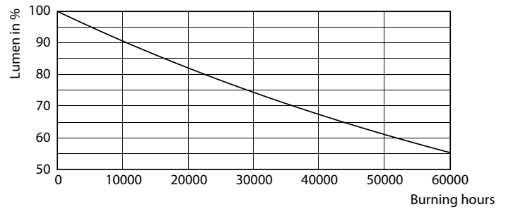
Lumen Maintenance Diagram - RS060B LED5-36/830 PSR II WH LILO
