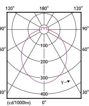
Light Distribution Diagram - Corepro LEDspot 550lm GU10 840 120D
