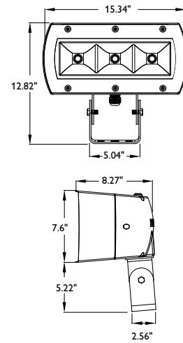
Trunion mount
