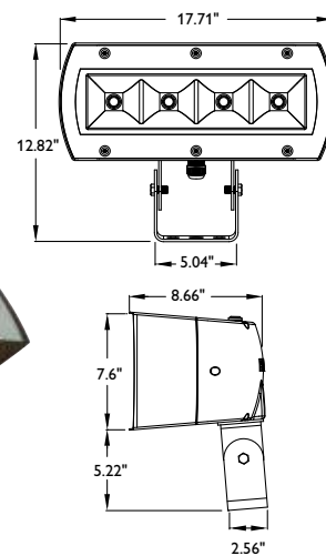
Trunion mount
