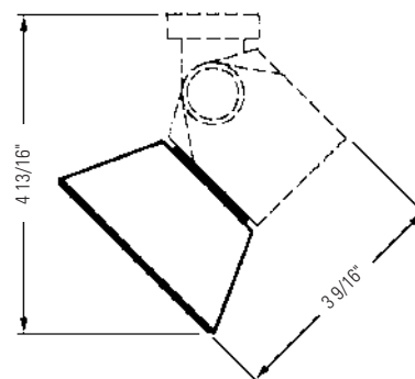
CONE 16 WITH HINGED ADAPTER
