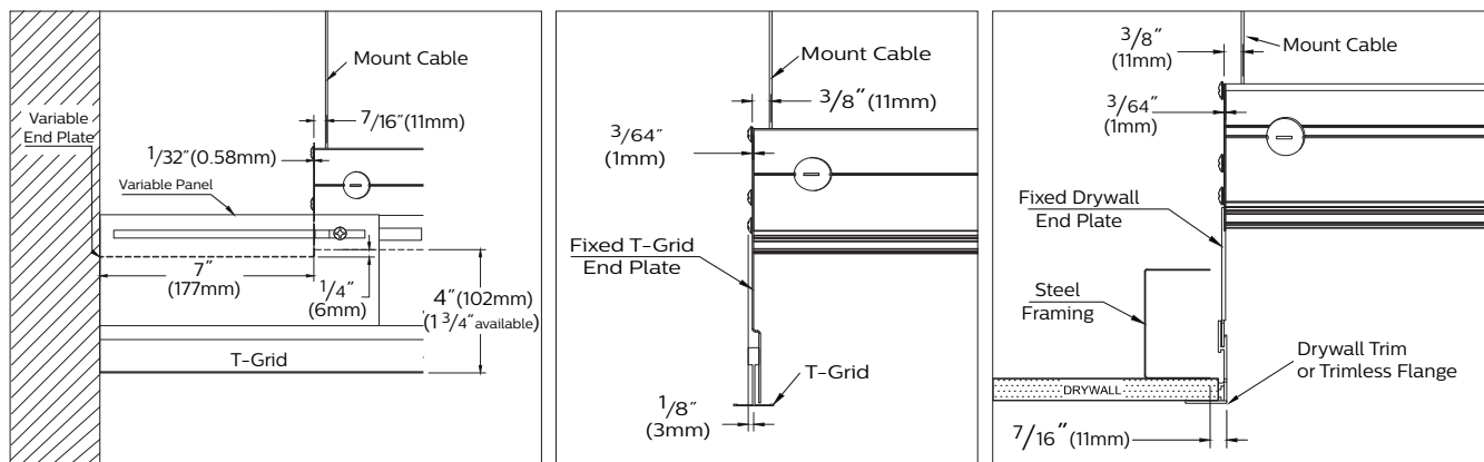
Variable/Wall End Set Detail T-Grid and Drywall
